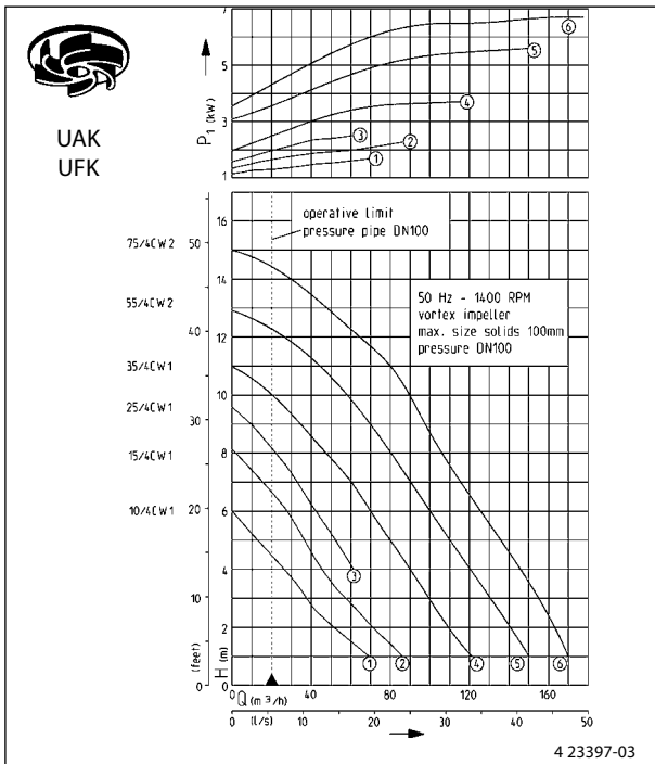
The minimum flow rate in the pressure pipe of v = 0,7 \text{ m/s} is marked in the Q-H-diagram (operative limit). Pump performance is subject to ISO 9906 tolerances
